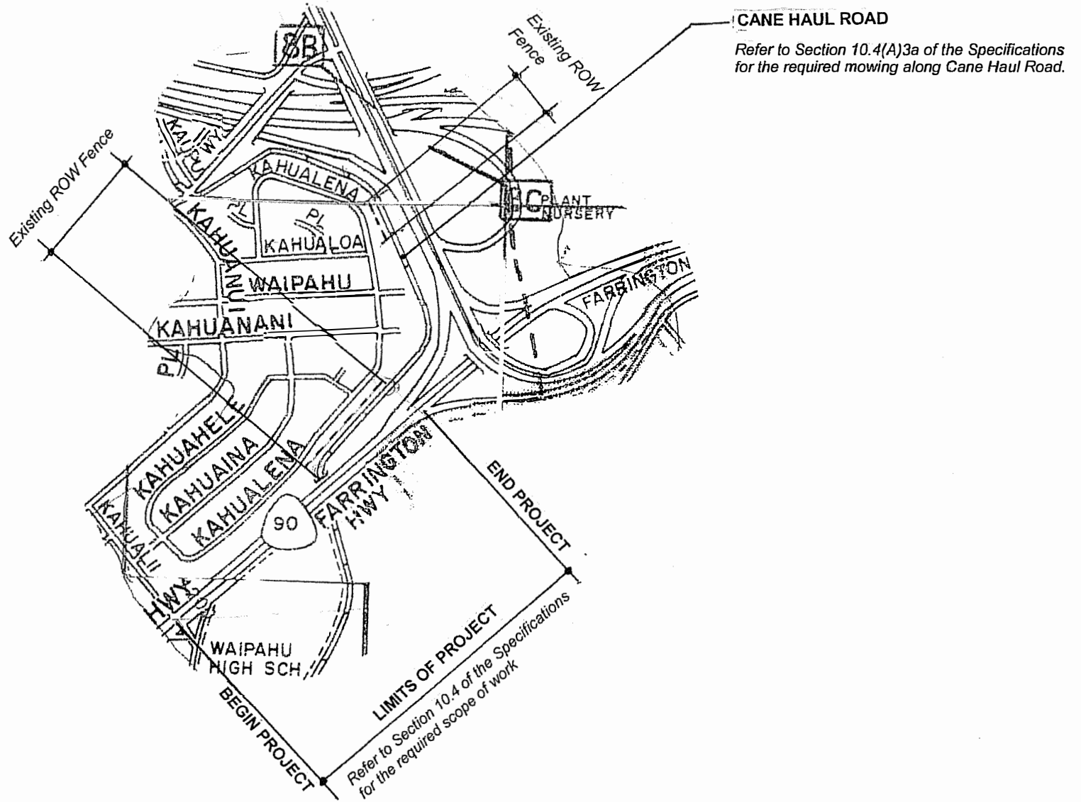
LOCATION PLAN ADDITIONAL RIGHT OF WAY AREA FARRINGTON HIGHWAY, KAHUALII STREET TO BEGINNING OF ON-RAMP, H-1 EAST BOUND PROJECT NO. H1D-01-24C(R) NOT TO SCALE
